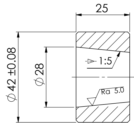
2 \sqrt{Ra 6.3} ( \sqrt{Ra 5.0} )
